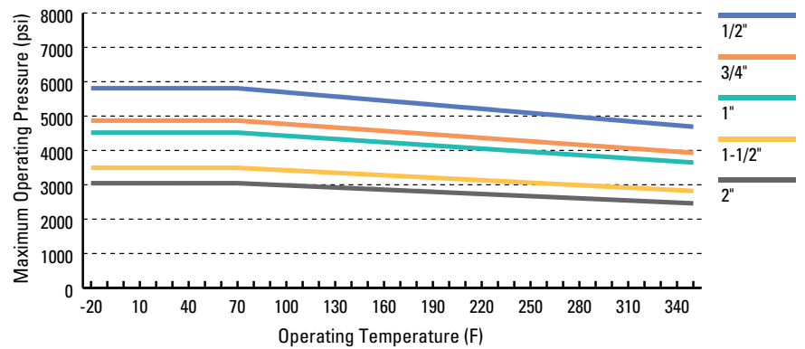
Monel 400 Male and Female NPT Fittings Pressure Ratings
