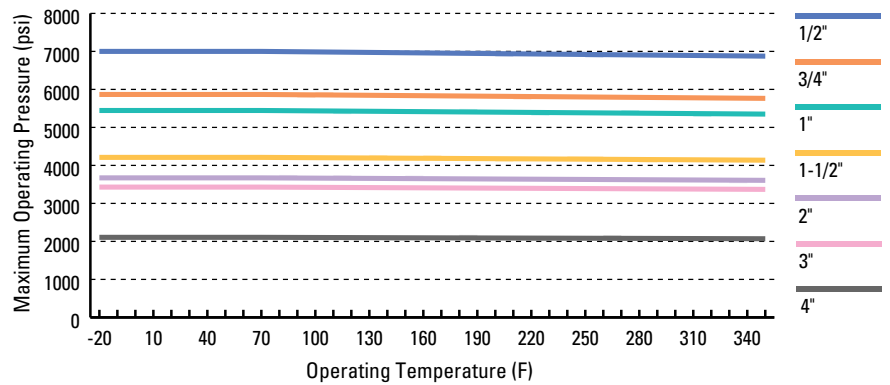
316 SS Male and Female NPT Fittings Pressure Ratings
